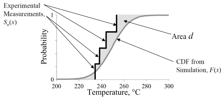
FIG. 4: Area validation metric example (reproduced from Ref. [23]).
