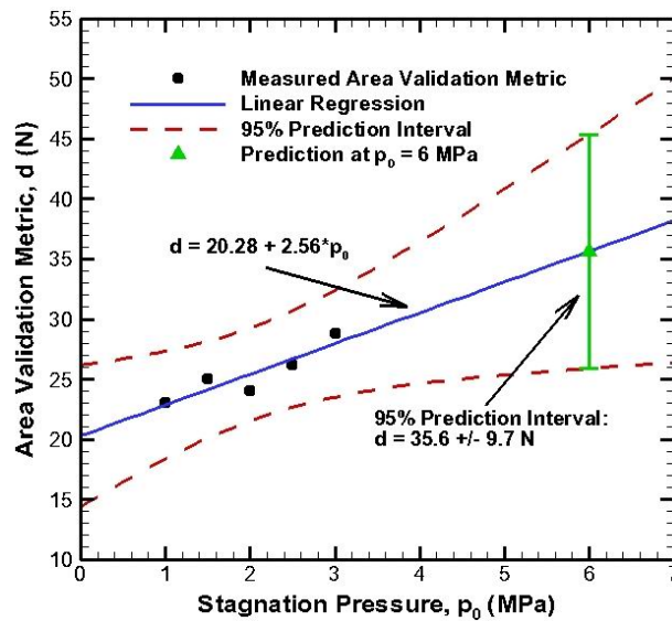
FIG. 11: Extrapolation of the area validation metric to the prediction conditions ( p_0 = 6 MPa) including prediction intervals.
