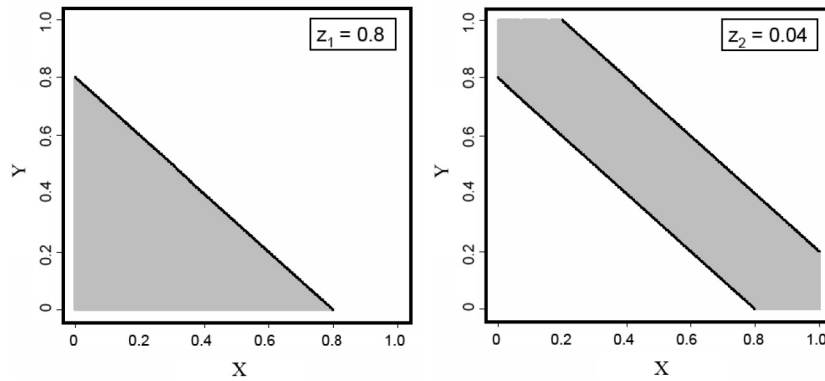
FIG. 5: Sets in the X - Y planes corresponding to sets Z \leq z .
