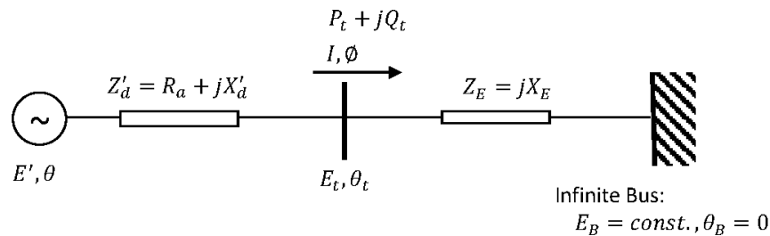
FIG. 1: Single machine infinite bus system.
