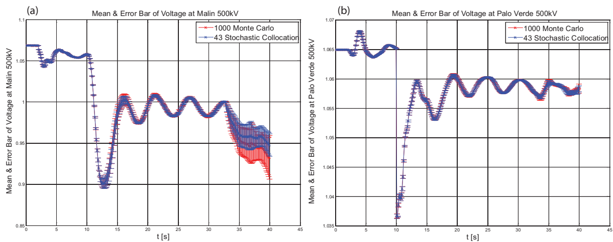
FIG. 11: Mean and error bar of voltage at (a) Malin 500 KV and (b) Palo Verde 500 KV using PCM on 43 sparse grid points and 1000 MC simulations.
